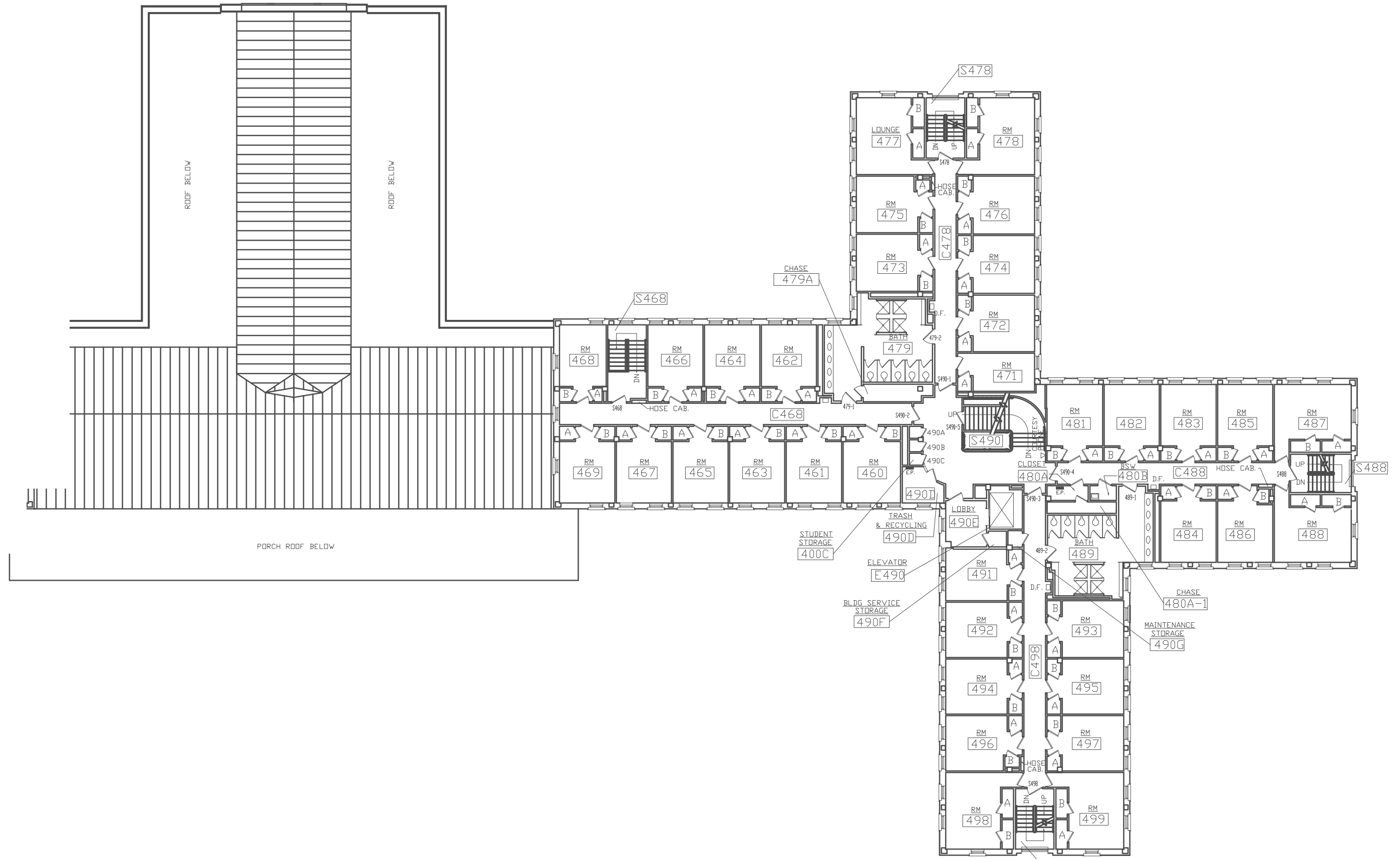
LEONARD HALL Fourth Floor Plan
