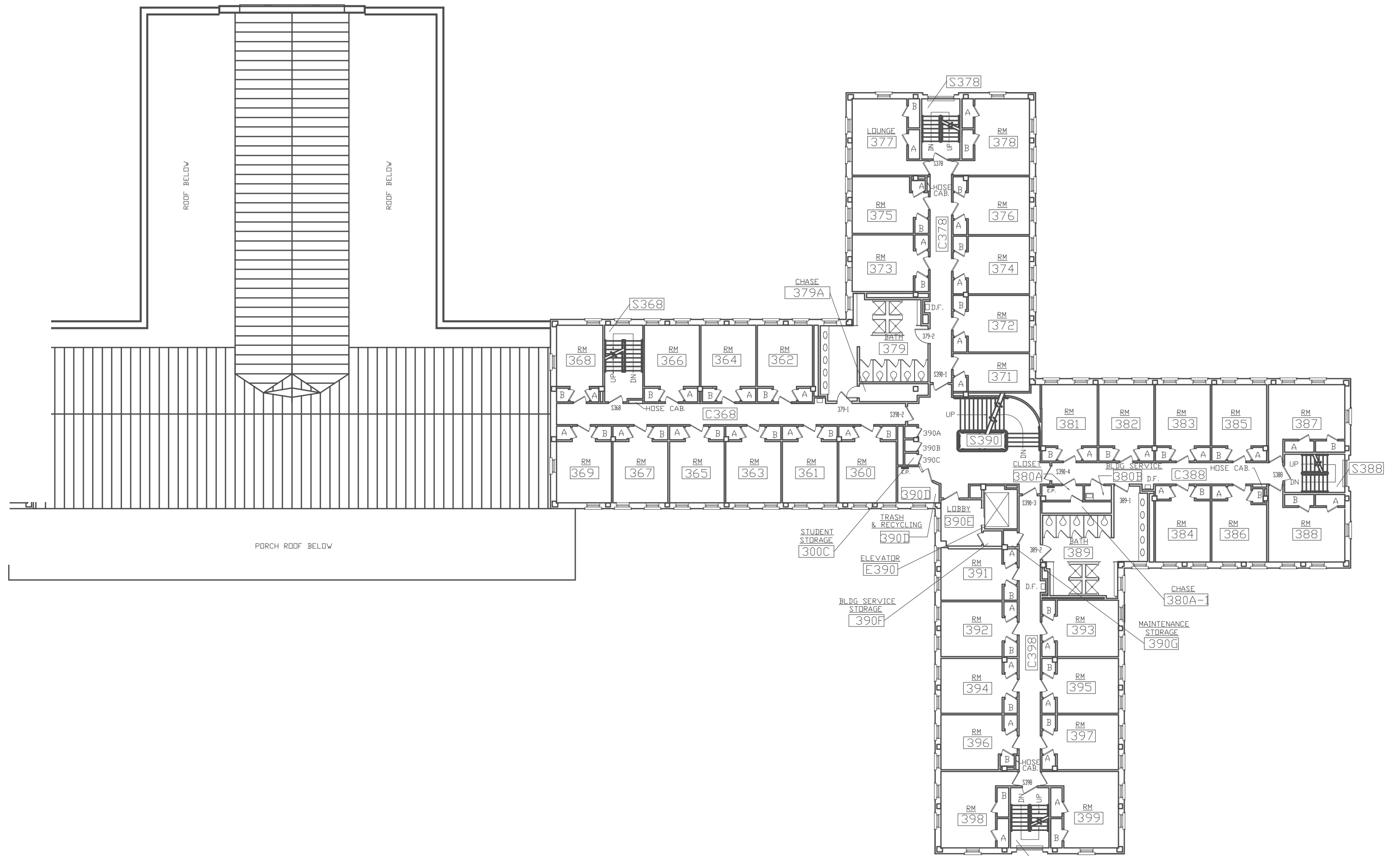
LEONARD HALL Third Floor Plan
